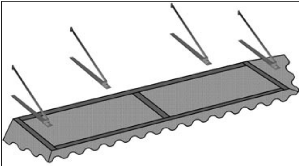
Oversized awning above is shown 'UP-SIDE DOWN' to illustrate additional support arm placement
