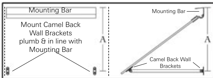
DOOR CANOPY MOUNTING CHART
